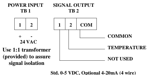
Figure 2.1 - Probe Terminal Connections
