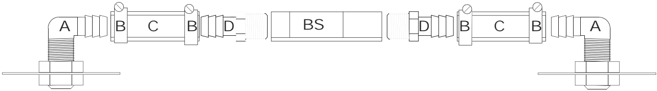
Figure 14. HB1/SB1 Ducted Damper Mount Detail View
