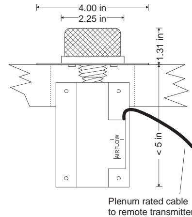
Figure 11. HB1/SB1 Floor Mount Installation Detail
