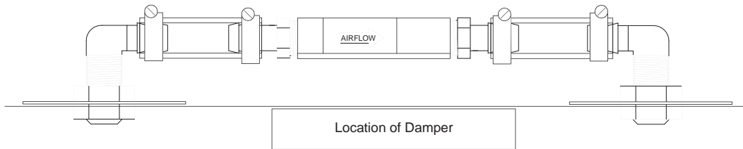
Figure 15. HB1/SB1 Ducted Damper Mount Installation Detail, Top View
