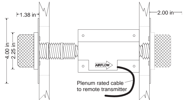
Figure 9. HB1/SB1 Wall Mount Installation Detail, Top View
