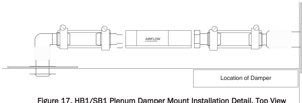
Figure 17. HB1/SB1 Plenum Damper Mount Installation Detail, Top View
